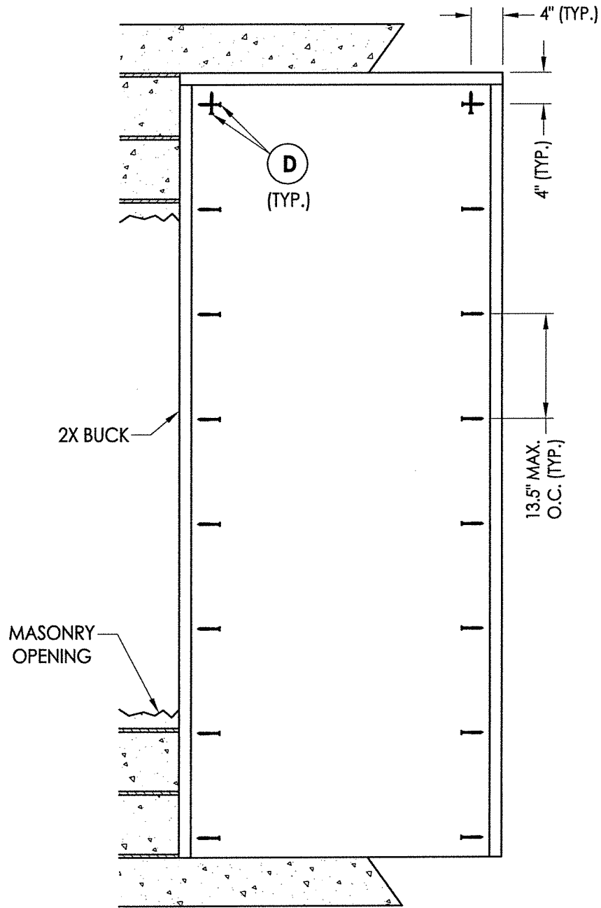
BUCK ANCHORING
