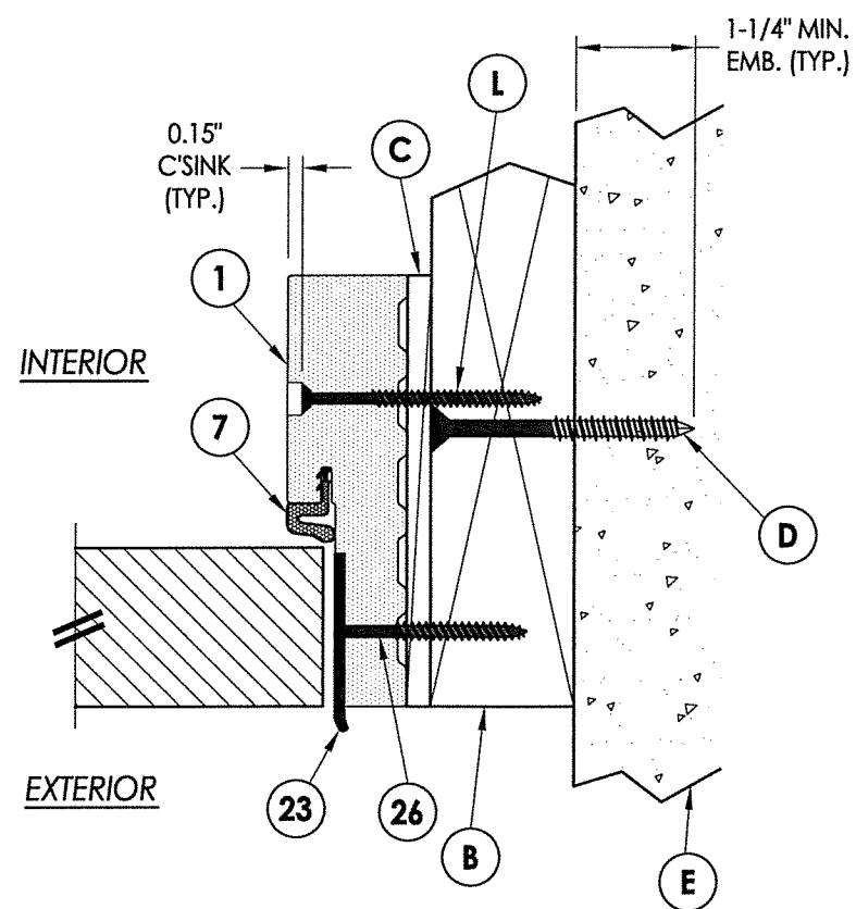
4 HORIZONTAL CROSS SECTION 3 2X Buck Construction
