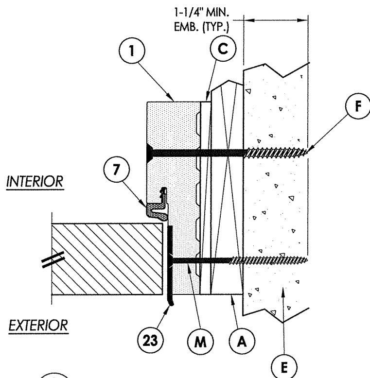
2 HORIZONTAL CROSS SECTION 3 Shown w/1X sub-buck
