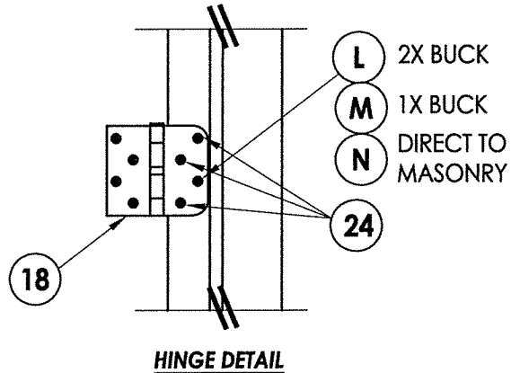
HINGE DETAIL
