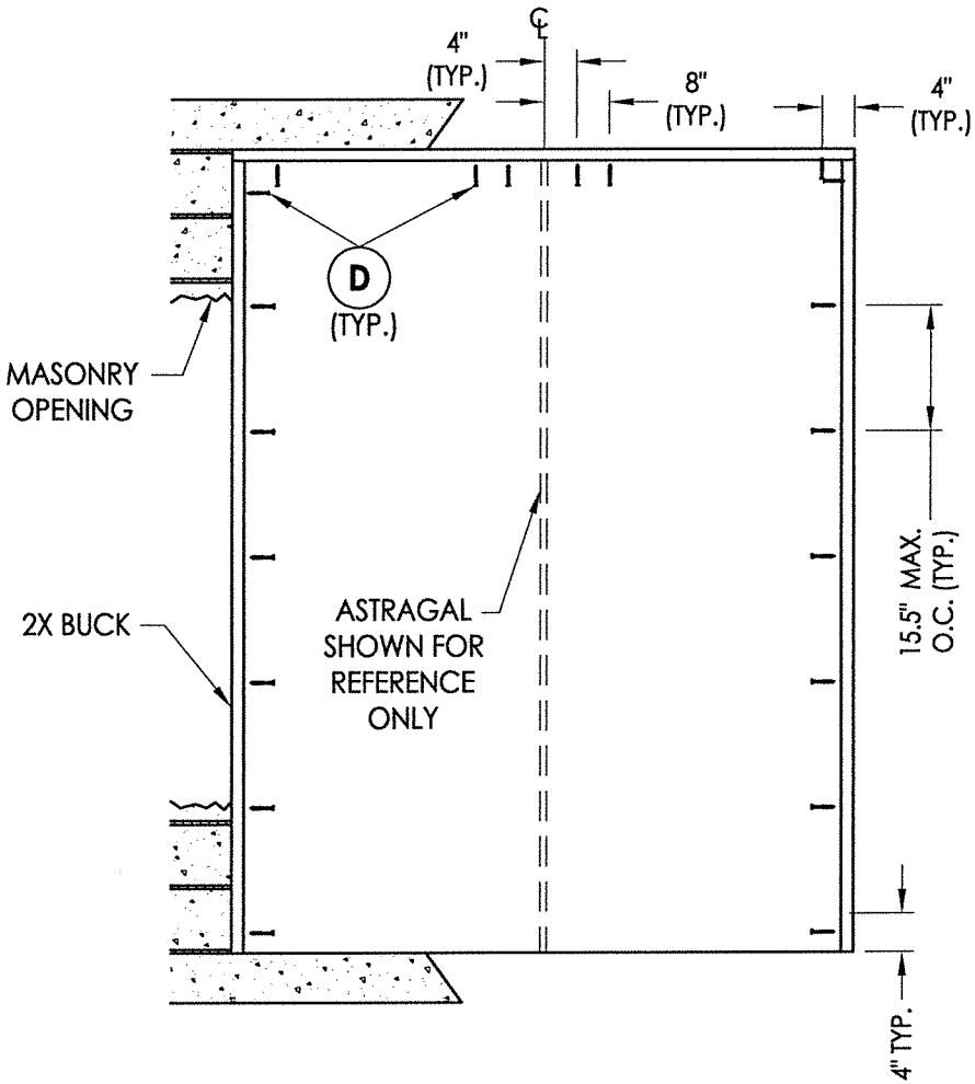
BUCK ANCHORING
