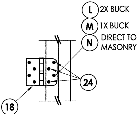
HINGE DETAIL
